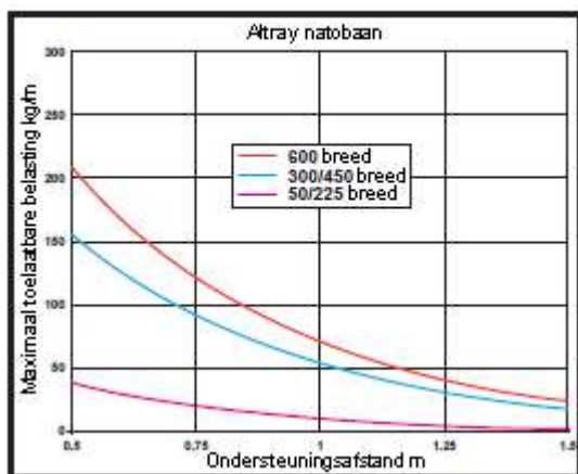
Belasting diagram
